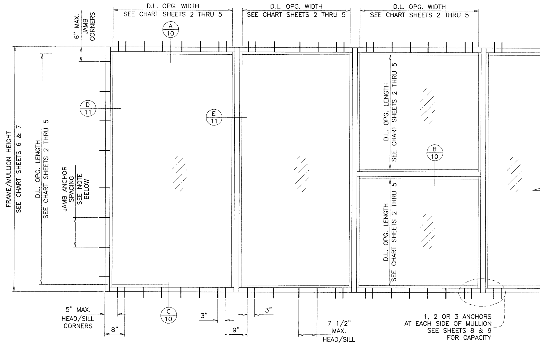
TYPICAL ELEVATIONS
