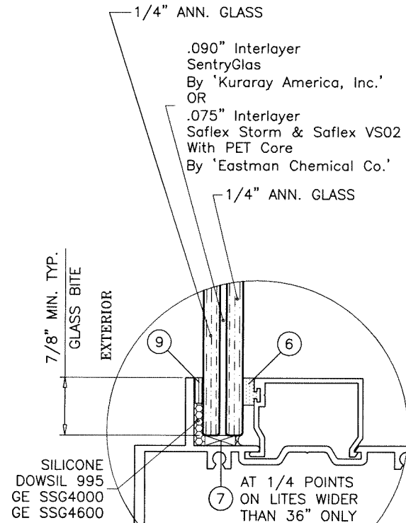
GLASS TYPE 'A' 9/16" OVERALL LAM. GLASS
